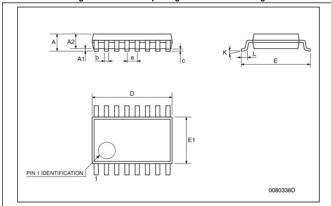
Figure 57. TSSOP16 package mechanical drawing
